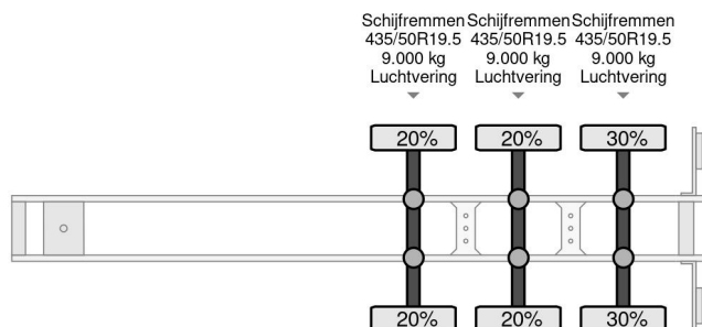
Samro ST39WJPA 3X BPW AXLE
