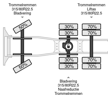
Scania T113-360 6X2 - MANUAL - FULL STEEL
