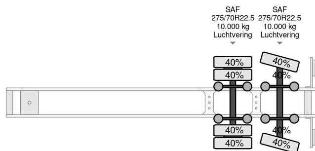
Kel-Berg S35-2 - CITYTRAILER + LAADKLEP + STEERING ...
