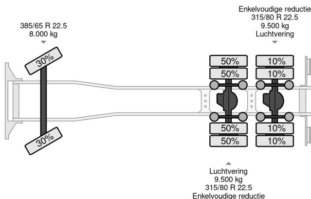
Scania R560 V8 6X4 Euro 5 CableLift
