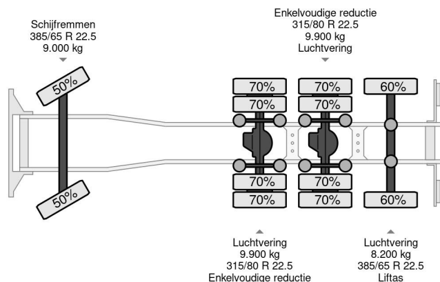
Scania R650 V8 8X4 RETARDER - CHASSIS
