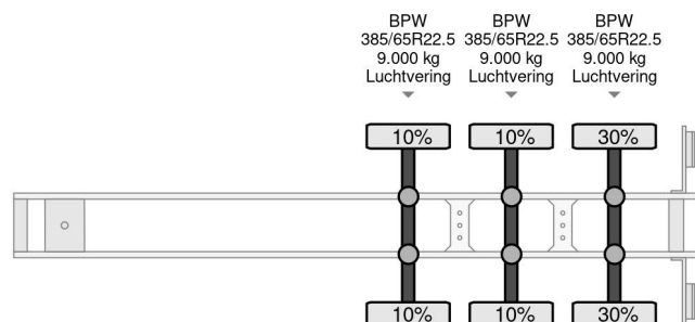
TURBO'S HOET KIPPER - 3 AXLE BPW + LIFTING AXLE + ...
