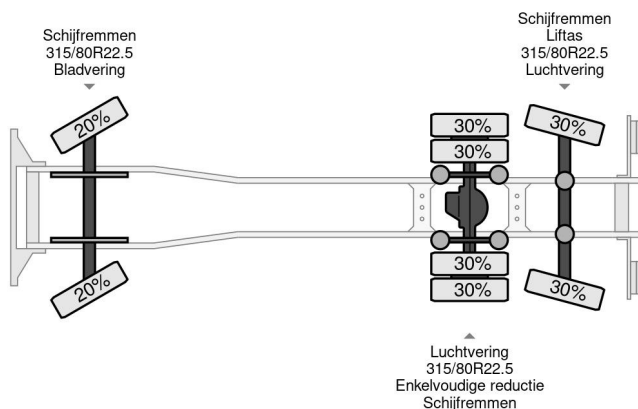
DAF CF 440 6X2 EURO 6 DALBY 20T
