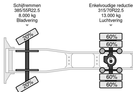
Volvo FM 330 4X2 - EURO 6 + AUTOMATIC + SKIRTS
