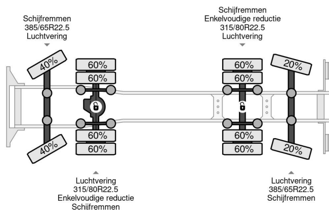
Volvo FM 500 8X4 HIAB 288 + REMOTE CONTROL 5T... 8x2 Referentienummer: VO783862-K
