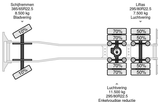
Scania R400 6X2 - EURO 5 + MULTILIFT HOOK + LIFTING ...
