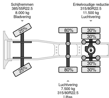
Volvo FH 460 6X2 - EURO 6 + LIFTING AXLE
