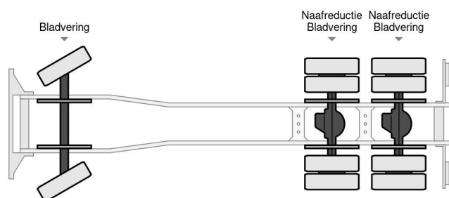
Scania T124-400 6X4 FULL STEEL MANUEL
