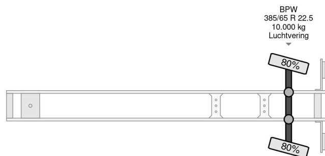
HMK BILCON 1 AXLE - ADR 26.600L - 5 COMPARTIMENTEN
