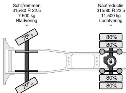
DAF XF 105.410 4X2 EURO 5 MANUAL + PALFINGER PK16...
