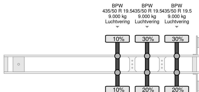
LAG 3 AXLE MEGA 1360x249x304
