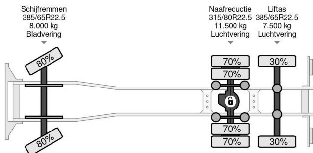
Scania P400 6X2 - EURO 5 + 3 CAMBER + LIFTING AXLE
