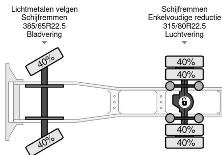
Scania T124-420 4X2 ORIGINAL 268803 KM
