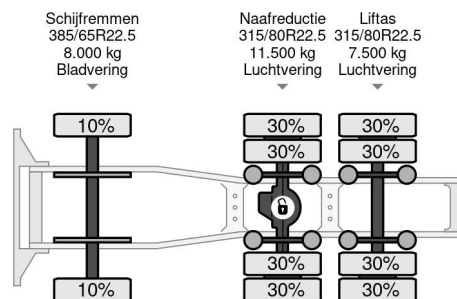
Volvo FH 540 6X2 - EURO 5 + BIG AXLE + LIFTING AXLE
