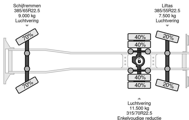
Volvo FH 460 6X2 PALFINGER PK53002 + REMOTE CONT...
