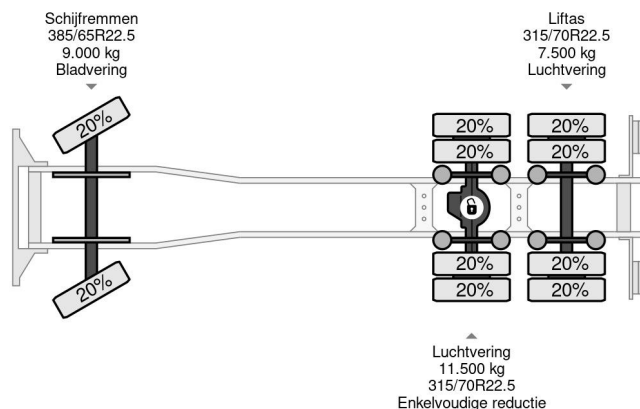
Volvo FM 370 6X2 EURO 6 VDL 21T HOOK
